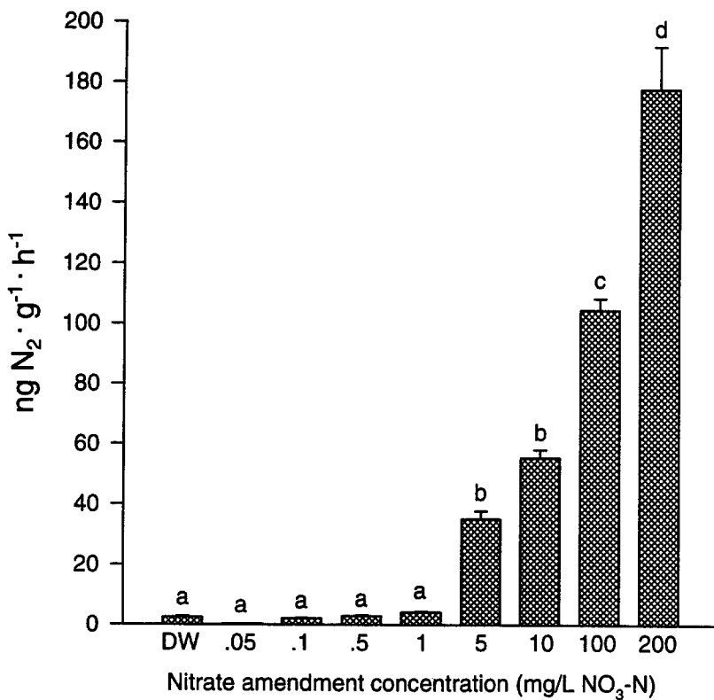
Figure 6. Effect of nitrate concentration on denitrification rate. All incubations were amended with 40 ml solution containing 3.3 g/L C as glucose and were incubated anaerobically. Error bars represent +1 SE, and statistically significant differences are indicated by different lower case letters.
