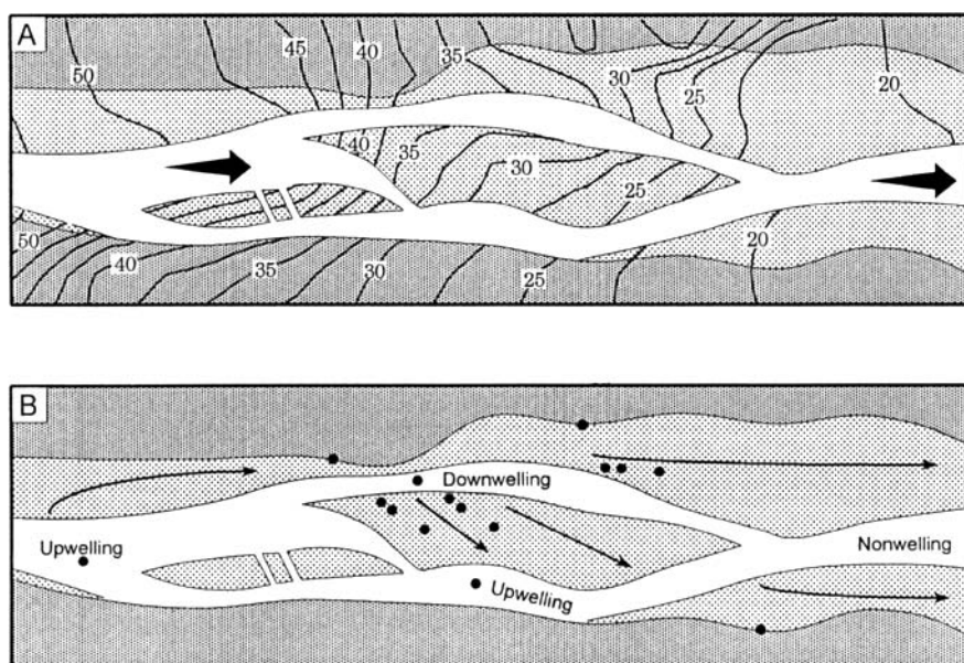
Figure 1. Overhead view of the study reach ( 100 \times 25 m). Unshaded region is the surface stream/hyporheic zone, lightly shaded area is the parafluvial zone, and darkly shaded region is the bank/riparian zone. A. Contour lines showing water table in parafluvial zone and bank sediments. Contour interval = 2.5 cm. Solid circles show typical sampling locations. B. Subsurface hydrologic flowpaths (determined by dye injections) and locations of hyporheic upwelling and downwelling.
