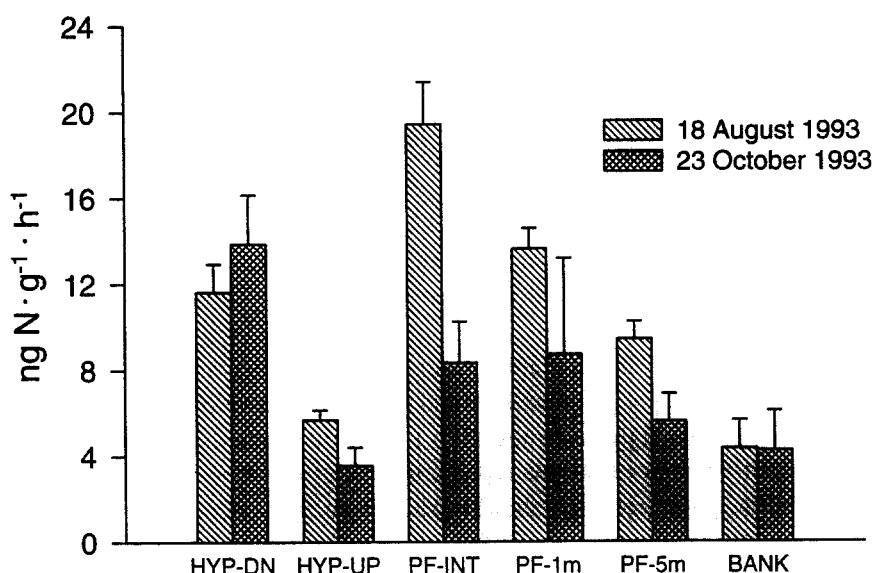
Figure 7. Net nitrification rate (per unit sediment dry mass). Error bars represent \pm 1 SE. Statistically significant differences among locations (Tukey's multiple comparison, p < 0.05 ) are denoted by different lower case letters.
